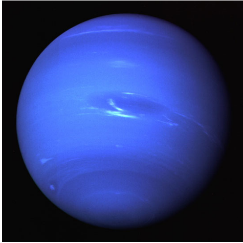
Neptune
